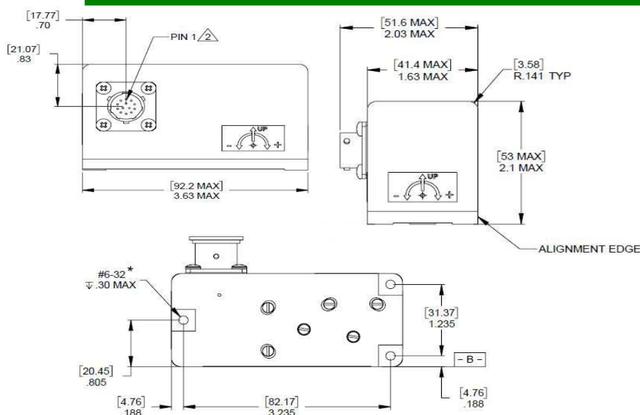
Dimensional Drawing: A750-200 Tiltmeter Series
