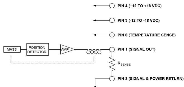
Pin Connections
