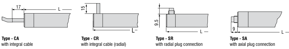
Type-CA with integral cable
