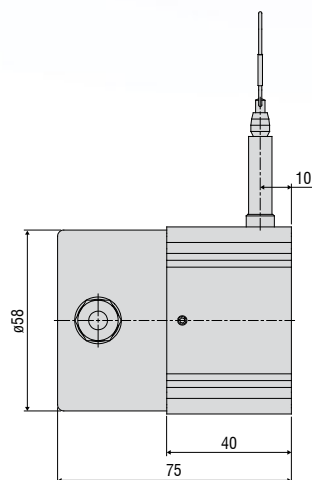
HTL/TTL output
