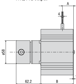
HTL/TTL output
