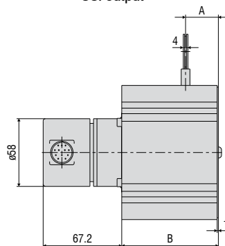
SSI output
