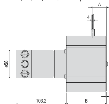
CO/PB/PN/ENIP/CAT output
