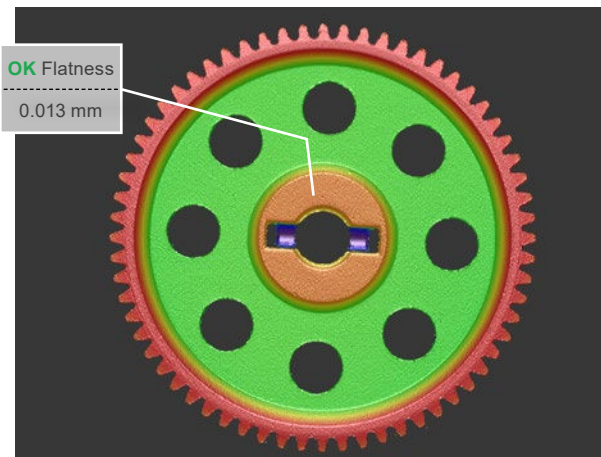
Flatness measurement of the flange of a gear wheel
